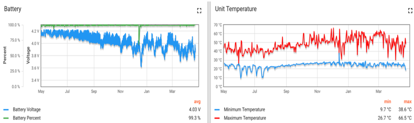
Figure 20. Indication of an overheating deck unit and the impact on battery voltage.
