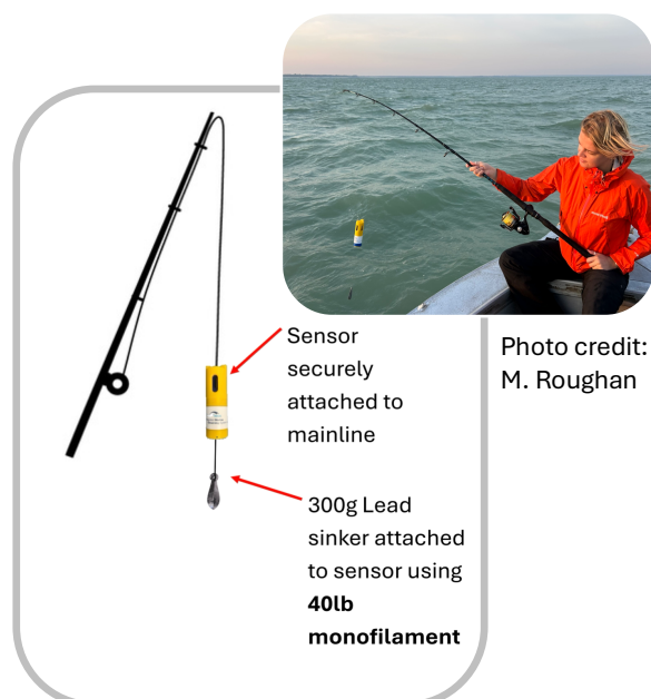
Figure 14. Moana sensor mounted to fishing rod schematic and photo.
