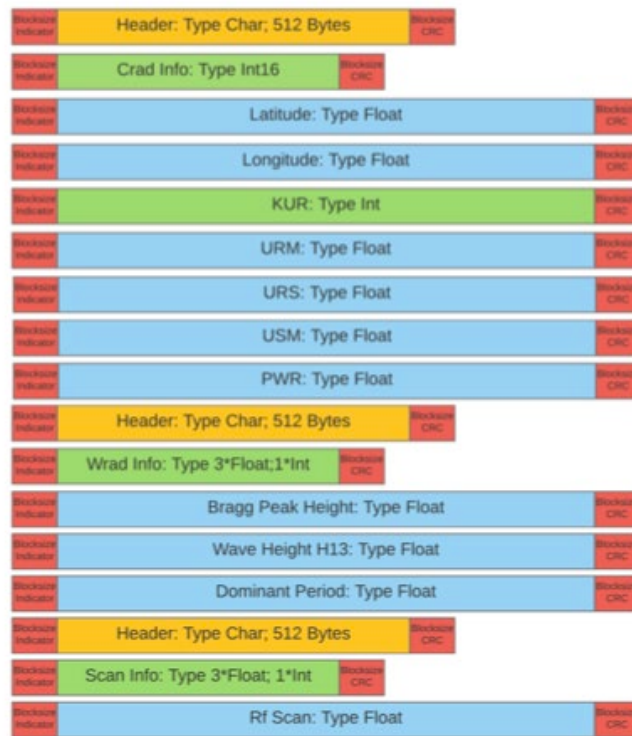
Figure 2. Structure of a WERA merged (radial, wave and frequency scan) binary file. The first block contains radial current information; single-radar wave information is stored in the second block. The third block contains a spectrum scan performed 2 minutes before the beginning of the acquisition cycle. WERA systems have the capabilities to dynamically adapt the operating frequency within the allocated frequency band, in attempt to decrease interference to normal operations. WERA HFRs managed by the IMOS Ocean Radar Facility however do not currently implement this feature.
