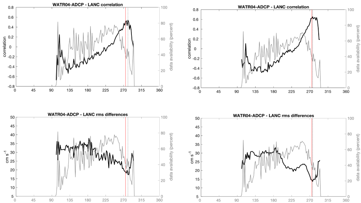
Figure 12. Example of the effects of RT QC FV00 applied to LANC radials on bearing errors. Left panel refers to RT FV00 without quality control; right panel refers to RT FV01 with quality control. Statistically significant improvement in correlation magnitude and rms differences can be observed when comparing RT data and DM QC FV01 data against current meter data.
