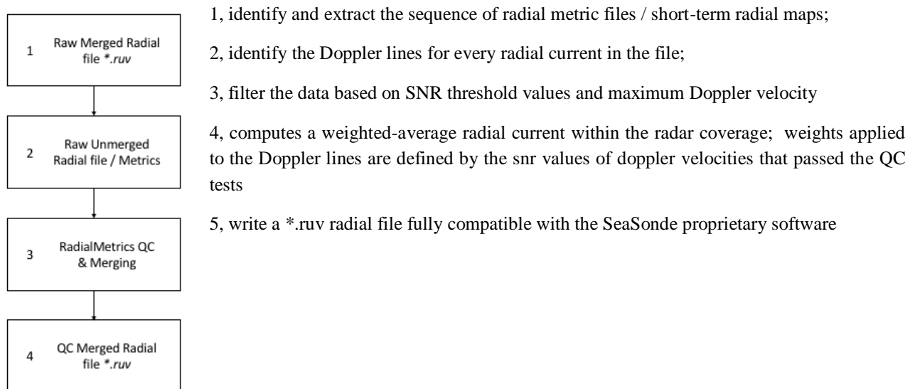
Figure 10. Flowchart of the proposed DM QC chain for the SeaSonde radial maps
