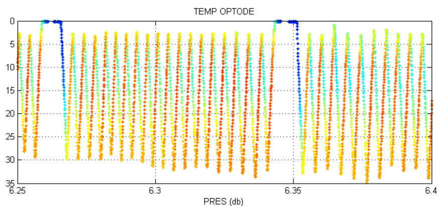
Figure 9 A sample temperature (°C) time-series data measured by the Optode during the June 2012 Storm Bay mission shows discrepancies between up- and down-casts.
