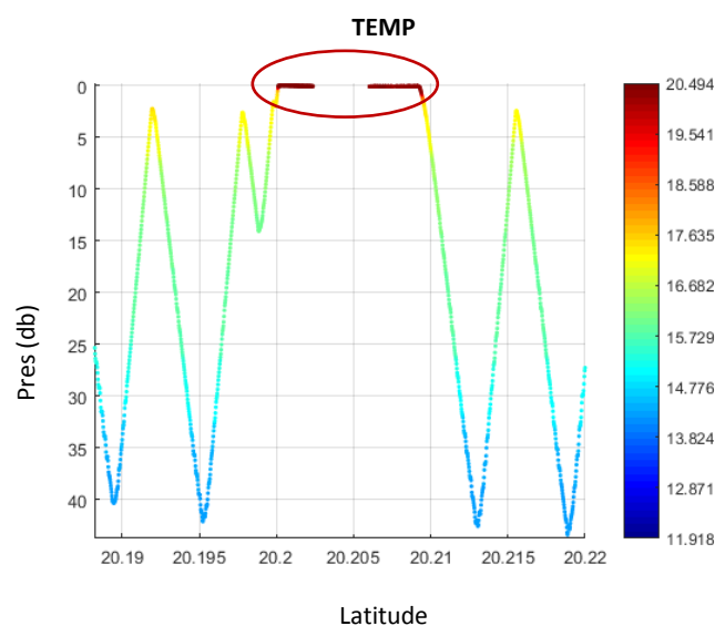
Figure 29 Significant raise in temperature (°C) recorded due to vehical heating while partly out of the water in surface parked position.
