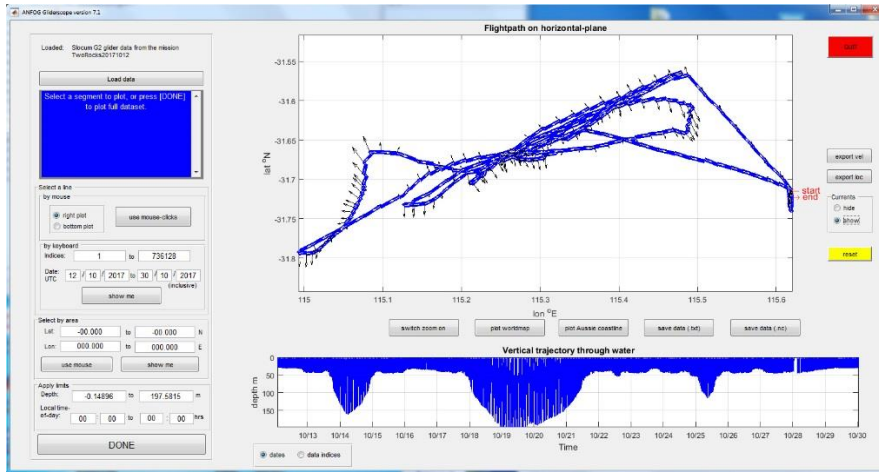
Figure 37 GLIDERSCOPE allows users to view the glider path and water velocity, as well as to isolate any segment of data spatially and temporally for visualisation/data export.
