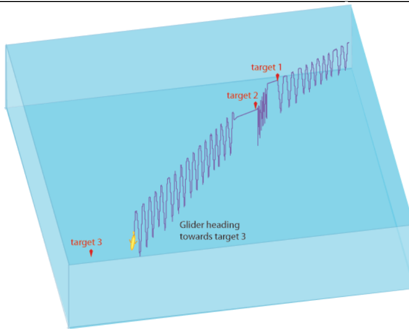
Figure 2. A Slocum glider performing 3 segments of saw-tooth lines. It surfaces at target points. This is different from a Seaglider, which usually surfaces after every descent-ascent cycle.
